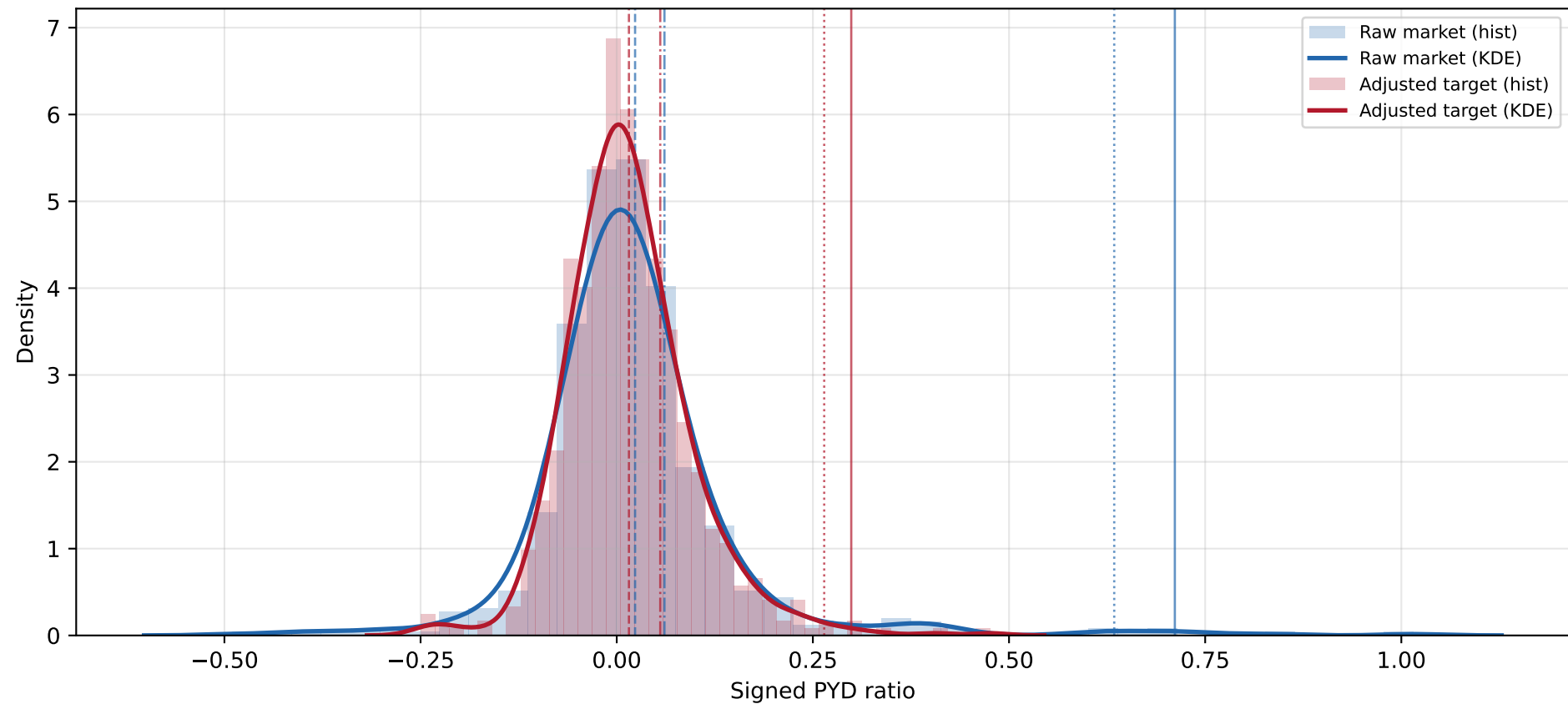
Distribution of signed PYD ratio Donor pool: FULL subset, n=674, adverse=367
