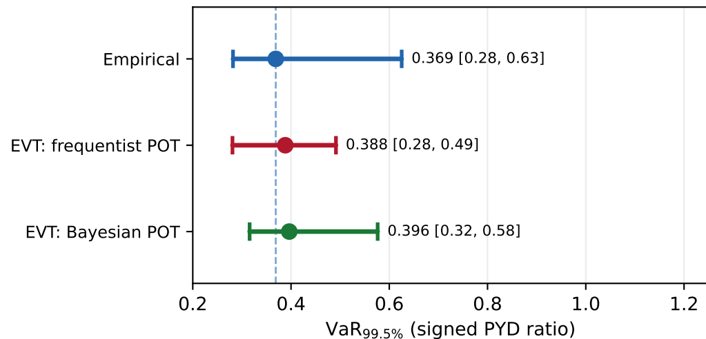
V2 (new profile) ( \hat{\xi} \approx 0.28 )
