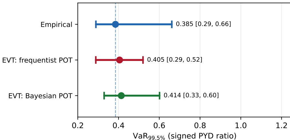
V1 (adjusted) ( \hat{\xi} \approx 0.28 )
