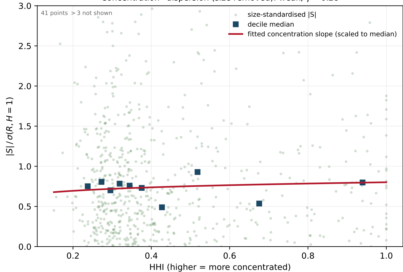
Concentration–dispersion (size removed): weak, \gamma = 0.28
