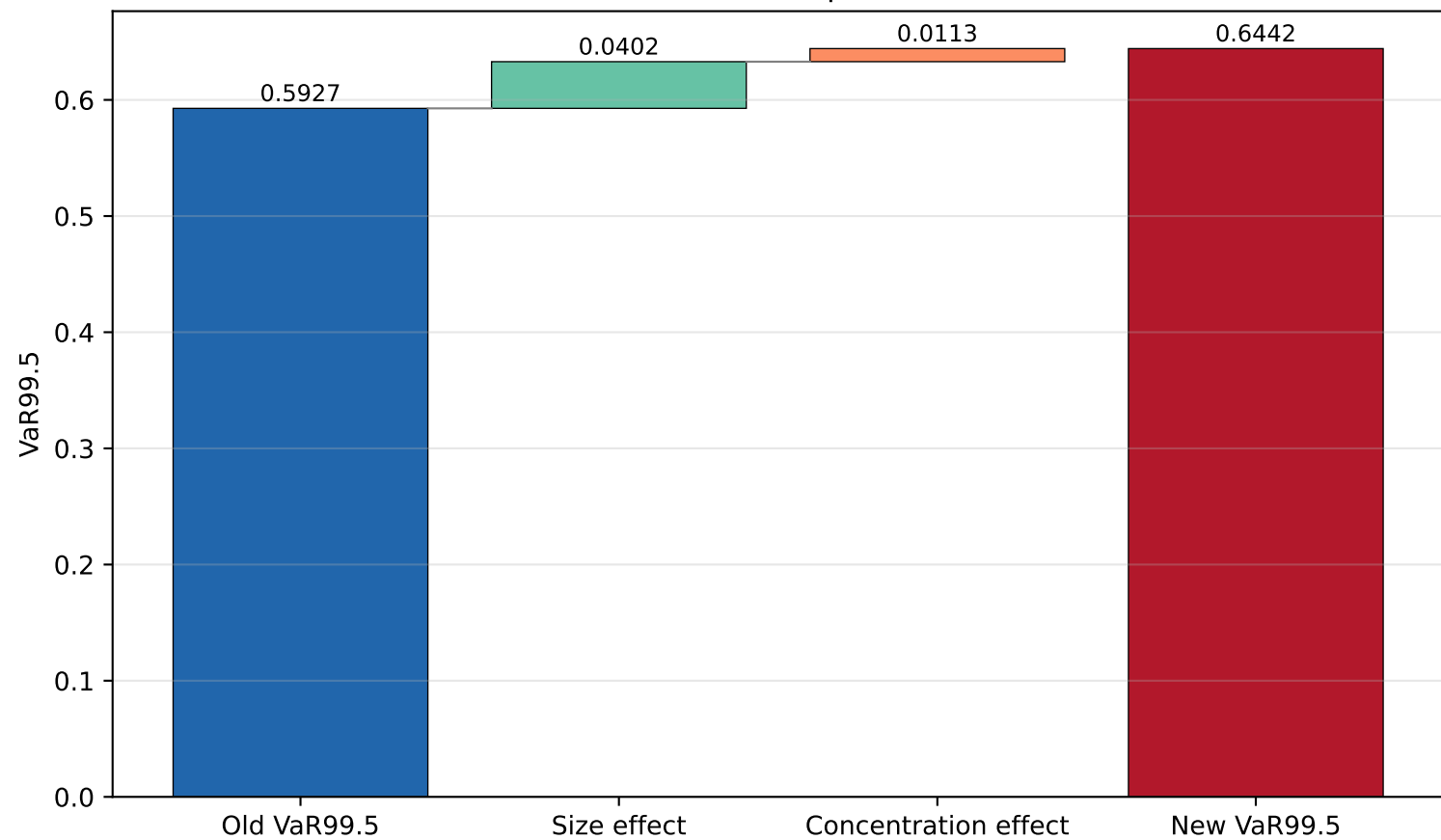
Profile transition decomposition: VaR99.5
