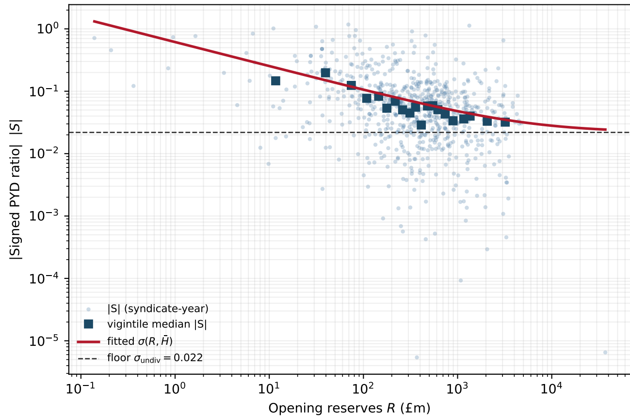
Size–dispersion: |S| decays with size toward the floor ( k = 0.61 )
