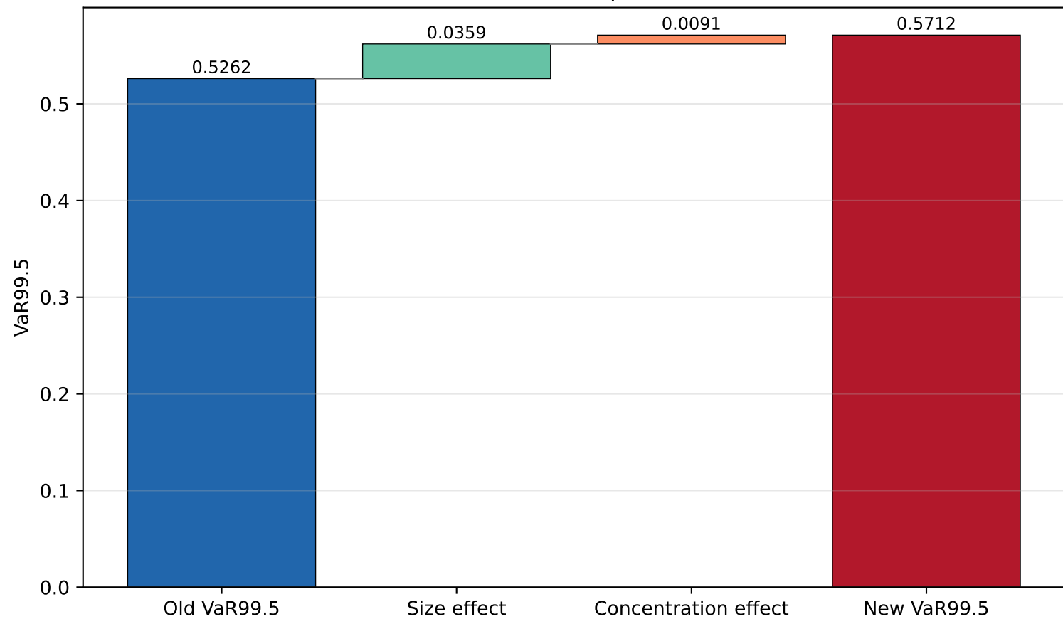
Profile transition decomposition: VaR99.5
