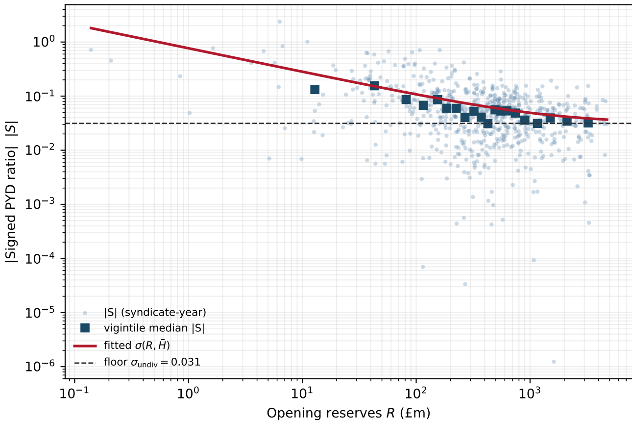
Size–dispersion: |S| decays with size toward the floor ( k = 0.56 )
