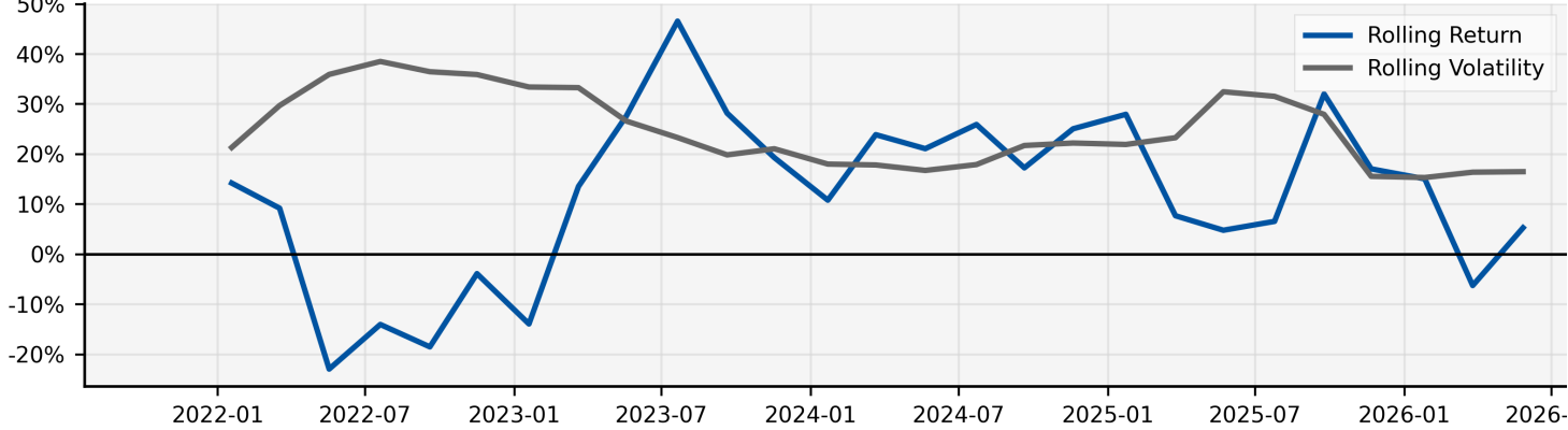
Rolling Stats [126 daily samples]
