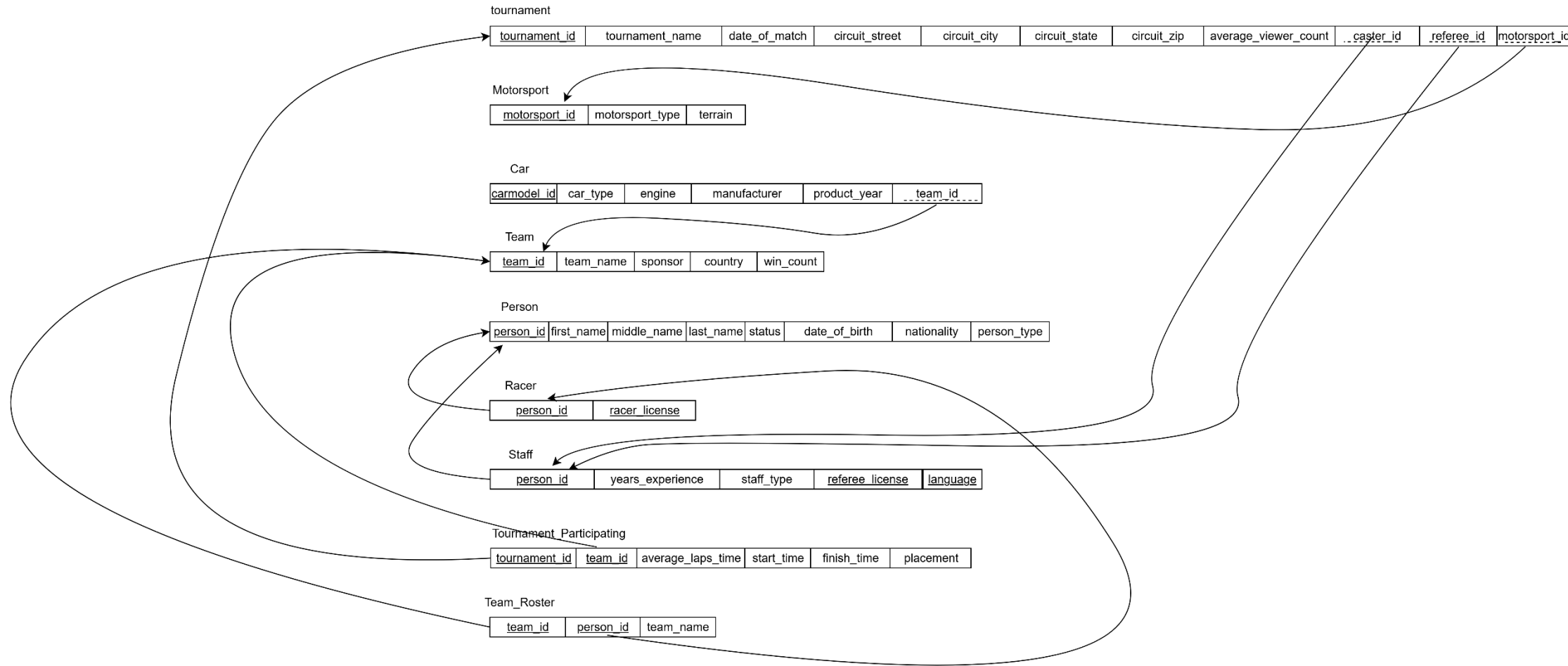
tournament
