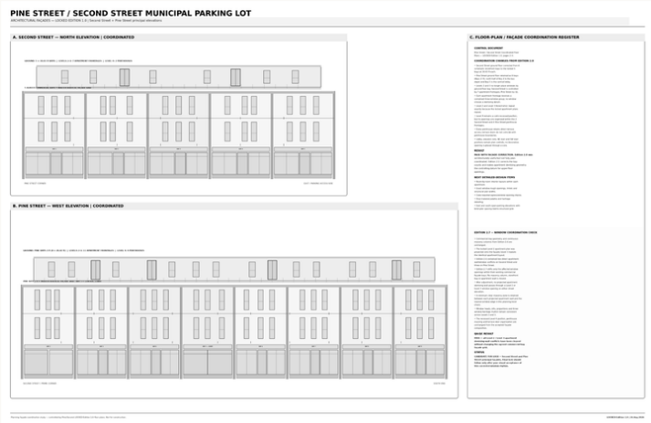
Controlled Second Street and Pine Street elevations.
