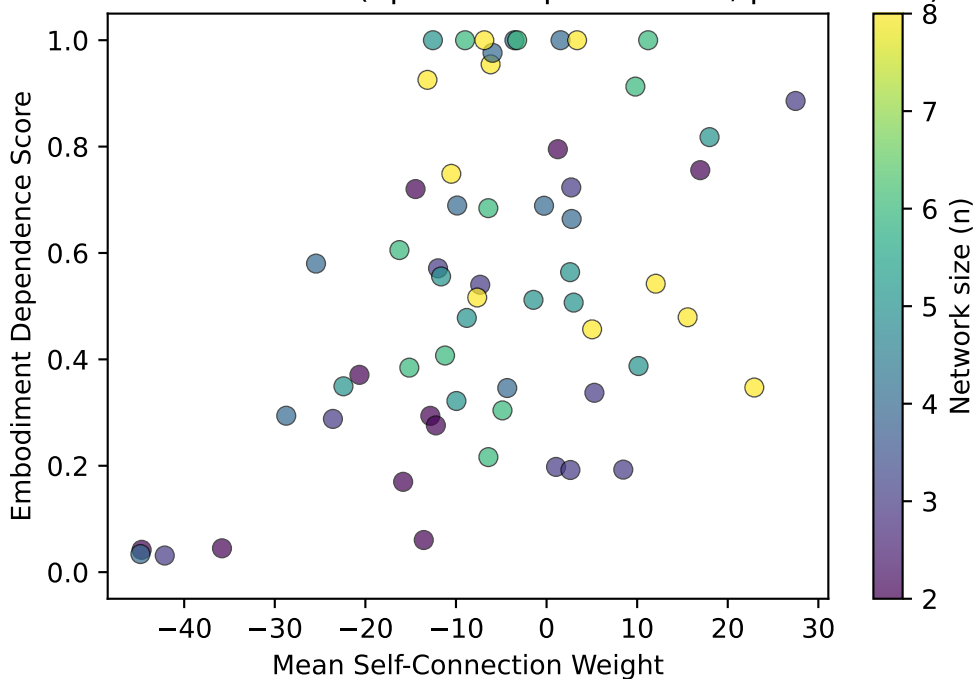
Self-Connection vs ED (Spearman \rho = +0.369 , p = 0.0037 )
