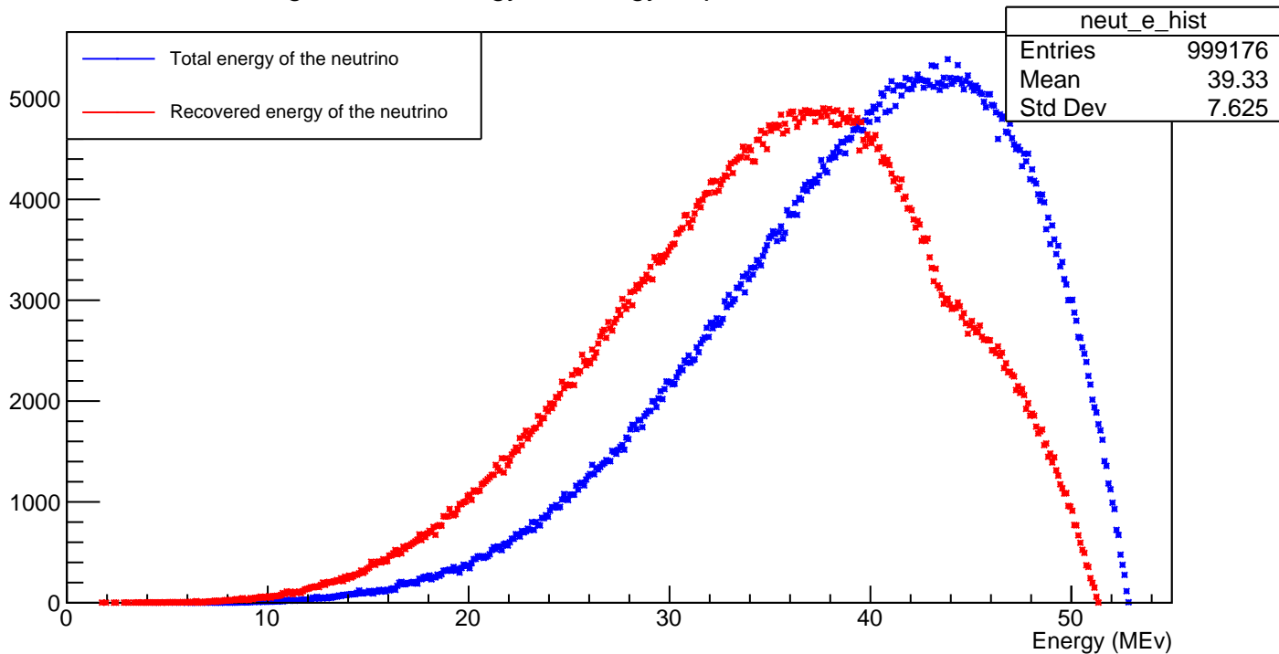
Incoming neutrino energy vs energy deposited in the TPC volume
