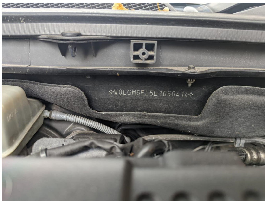
ClientVINjpeg-V1.jpeg
