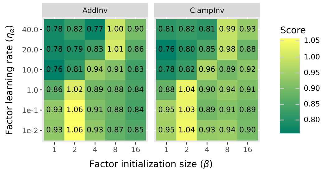
Concept score
