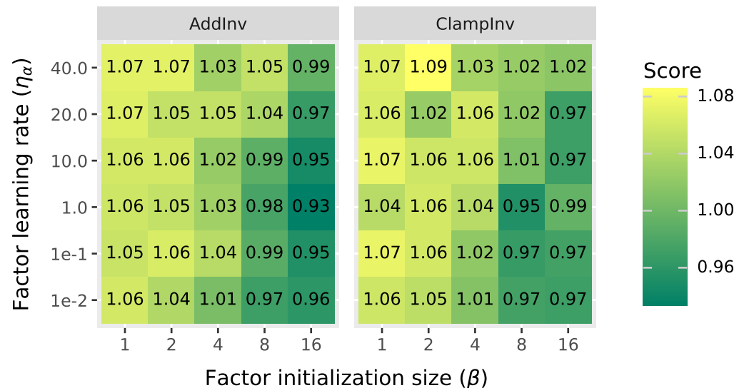
Fluency score
