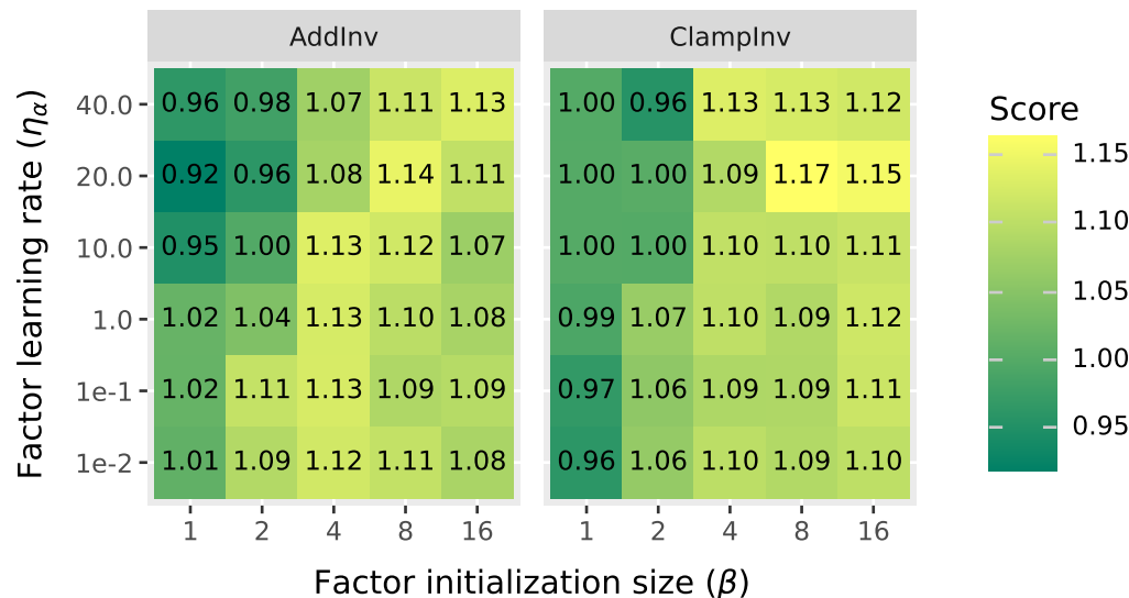
Overall score
