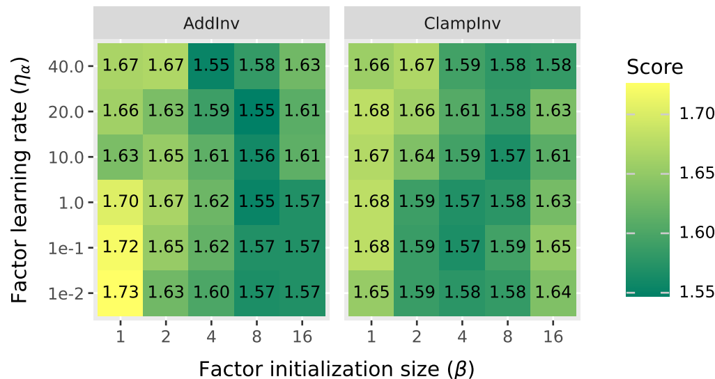
Instruct score
