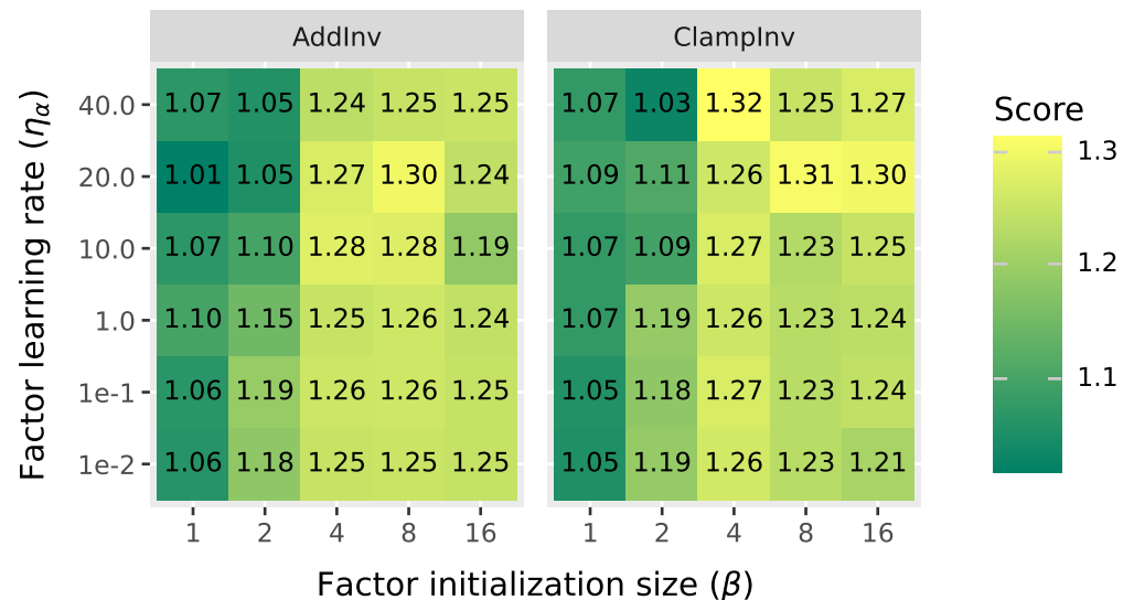
Concept score
