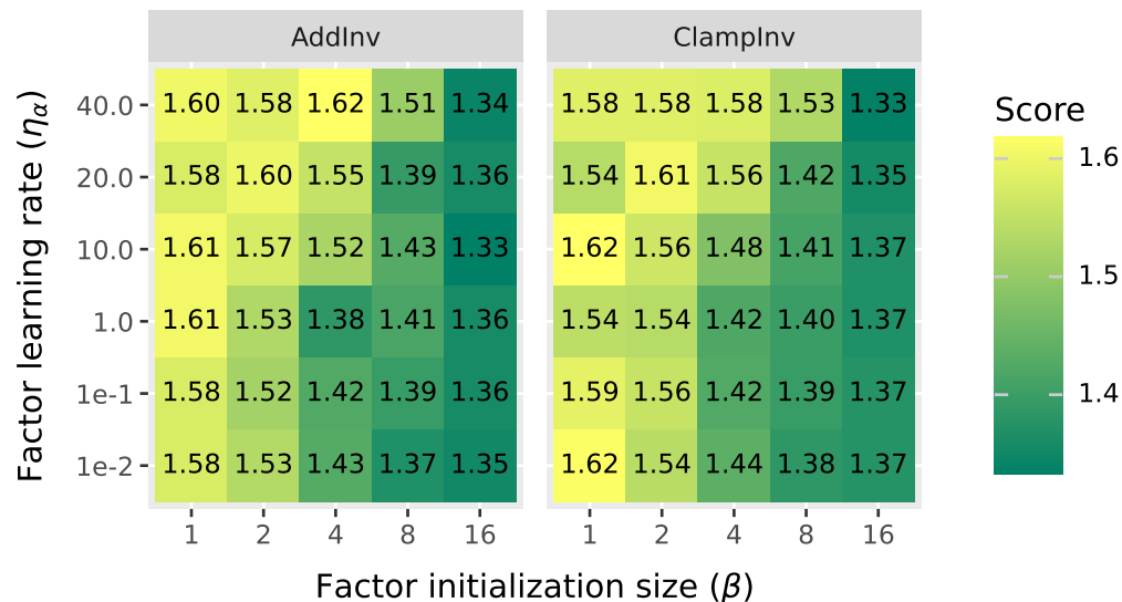
Instruct score
