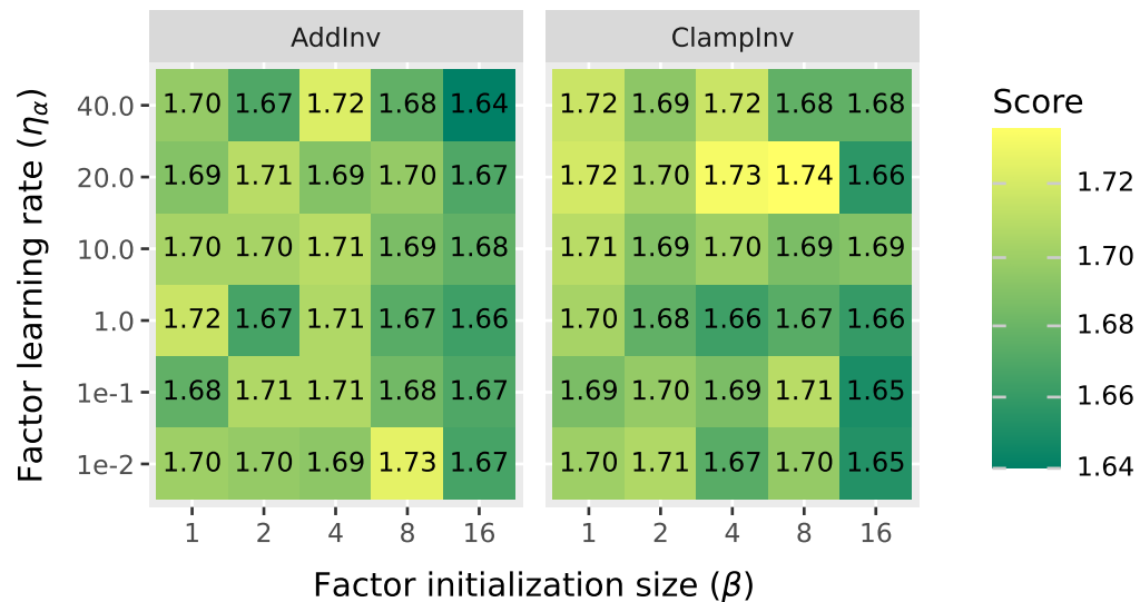
Instruct score
