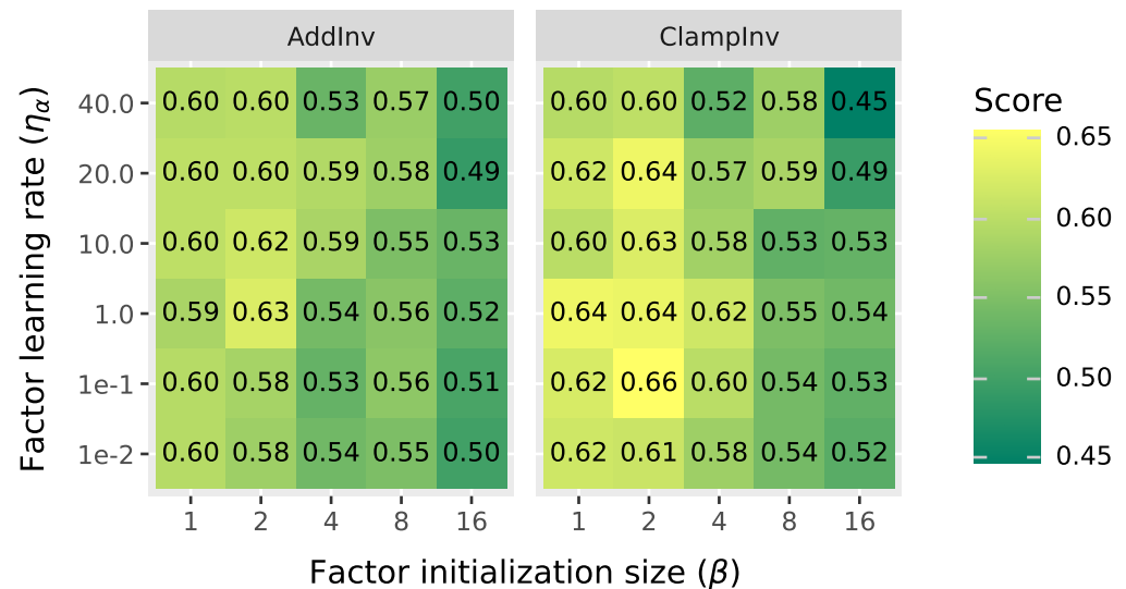
Concept score
