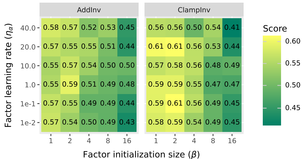
Overall score
