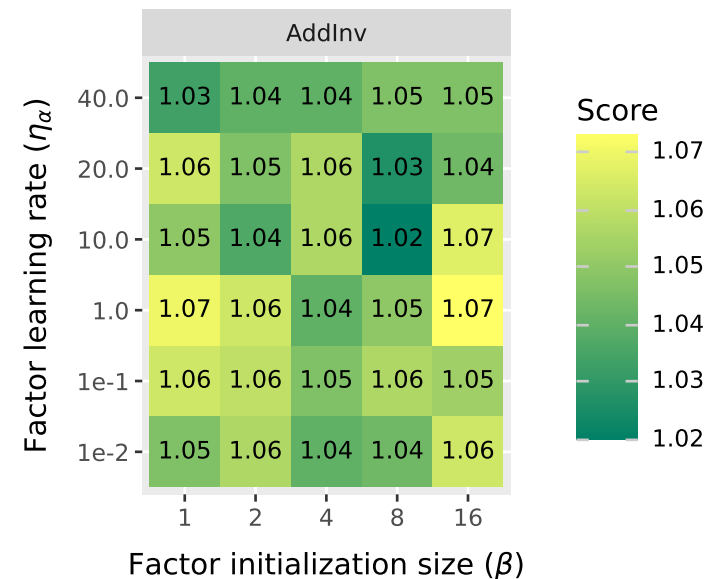
Fluency score
