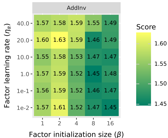
Instruct score
