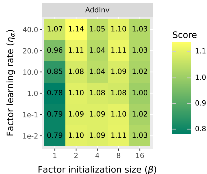
Fluency score
