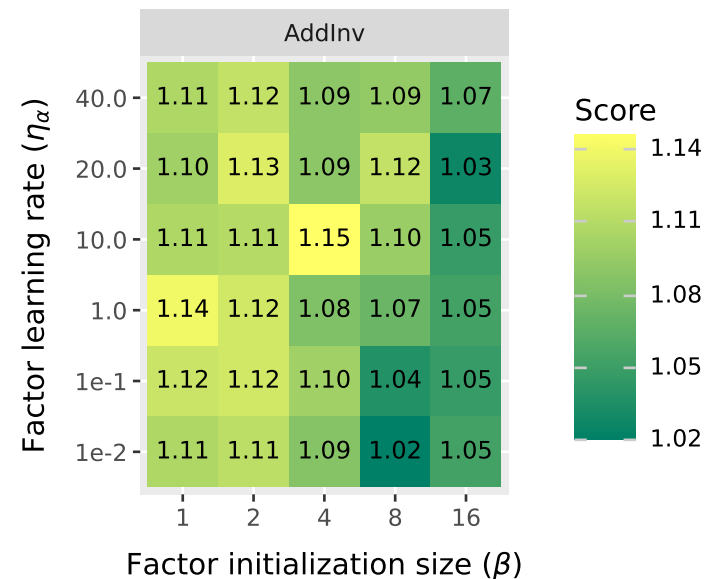
Fluency score
