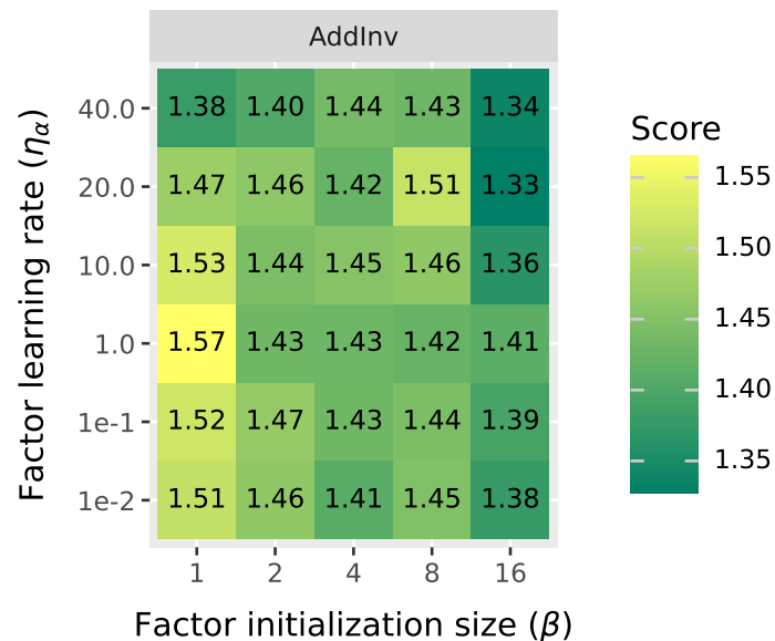
Instruct score
