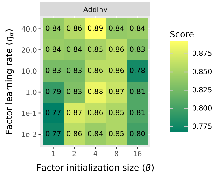
Concept score
