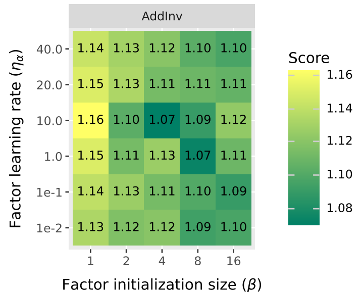
Fluency score
