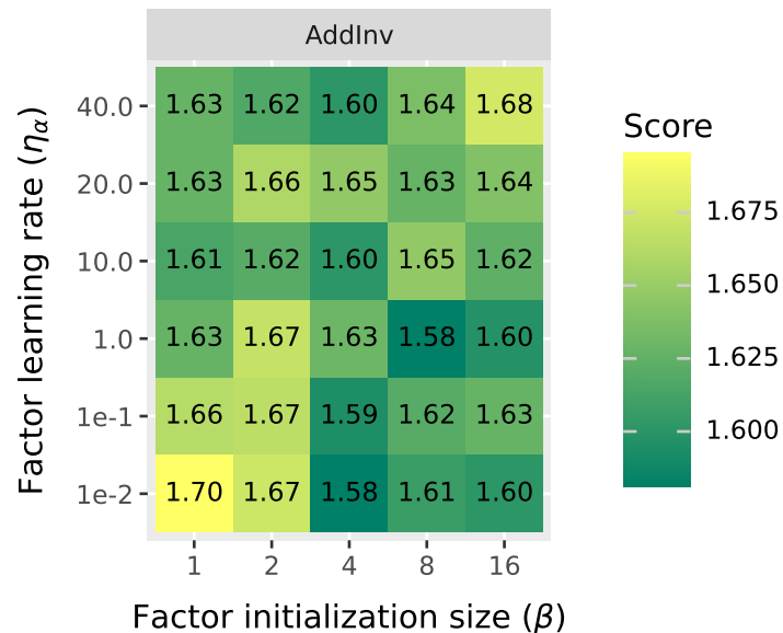
Instruct score
