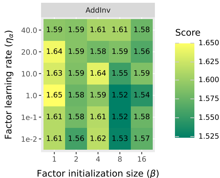
Instruct score
