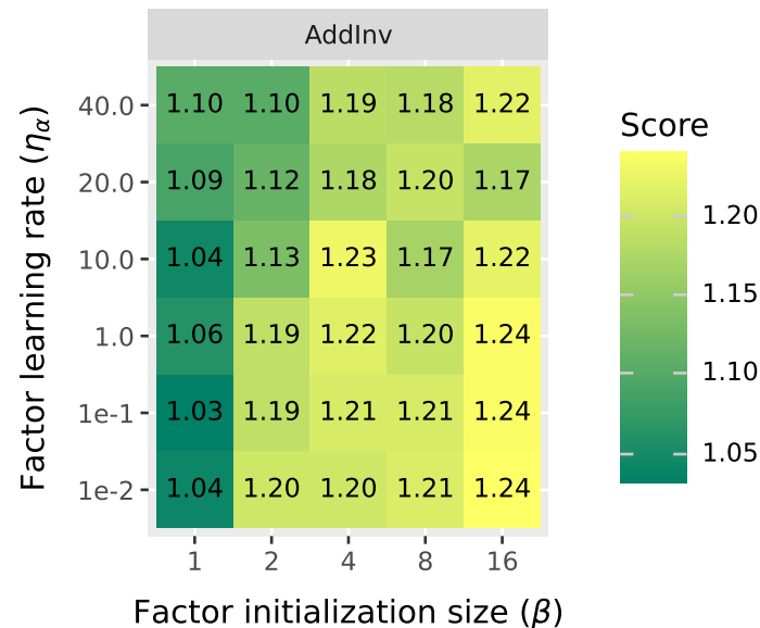
Fluency score
