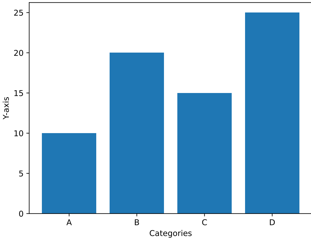
Bar Plot Example
