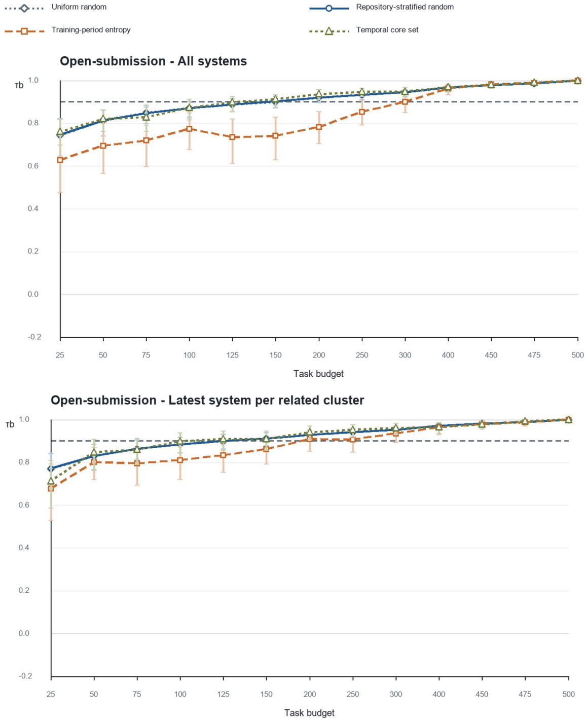
Fig. 2a Held-out Kendall's \tau_b by task budget and scope in the open-submission panel. The y-axis includes the full 0–1 fidelity range and extends to -0.2 so negative lower intervals remain visible. The dashed horizontal line is the primary mean threshold of 0.90; passing also requires the method-specific lower bound.
