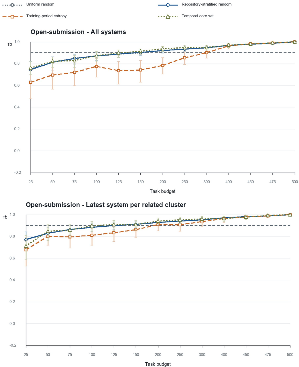
Fig. 2 (a) Held-out Kendall's \tau_b by task budget and scope in the open-submission panel The y-axis includes the full 0–1 fidelity range and extends to -0.2 so negative lower intervals remain visible. The dashed horizontal line is the primary mean threshold of 0.90; passing also requires the method-specific lower bound.
