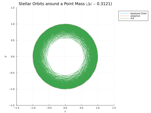
(f) RK4
