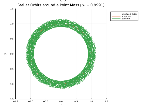
(h) Yoshida
