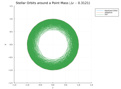
(f) RK4
