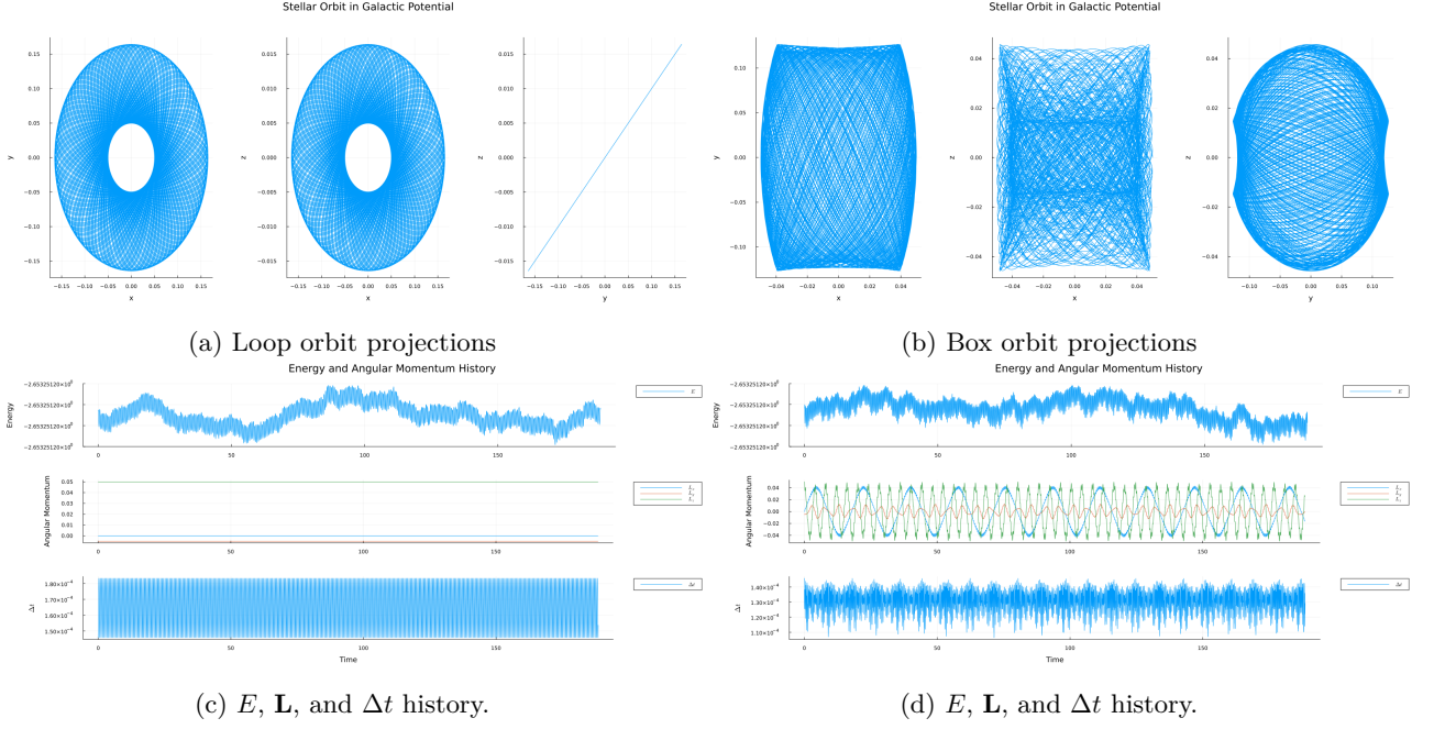
Figure 9: Comparison of box and loop orbits. The initial conditions are \mathbf{r} = [0.05, 0, 0] and \mathbf{v} = [0, 1.0, 0.1] . The loop orbit comes from a galactic potential with q_1 = q_2 = 1.0 . The box orbit comes from a galactic potential with q_1 = 0.75 and q_2 = 0.85 .
