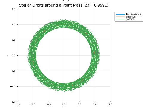
(h) Yoshida
