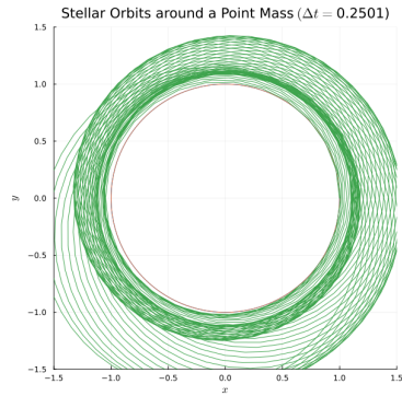
(e) RK2
