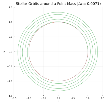
(a) Euler
