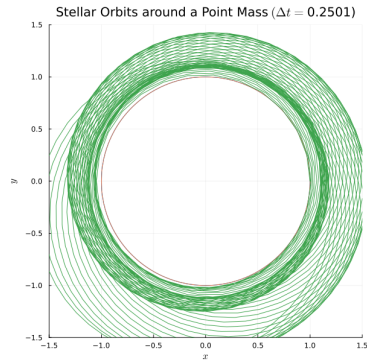
(e) RK2
