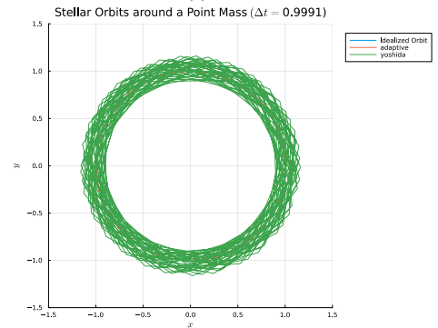
(h) Yoshida
