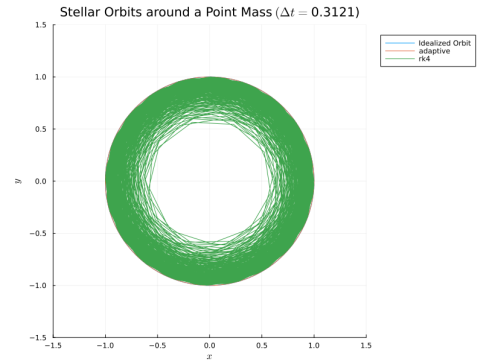
(f) RK4
