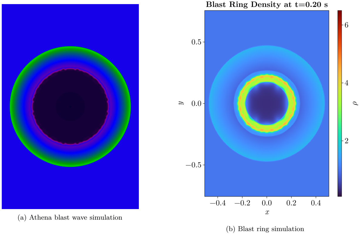
Figure 4: Comparison of Athena simulation and my simulation at t = 0.2\text{s} .
