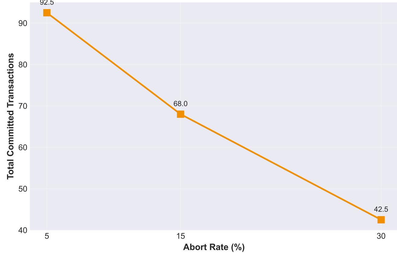
Throughput Degradation from Baseline (5%)
