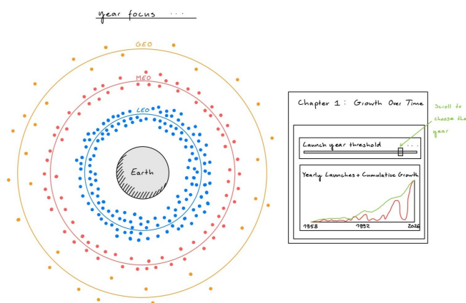
Figure 2. M2 wireframe — Growth Over Time . The intended structure: concentric orbital rings, a launch-year slider, and a yearly/cumulative chart beneath.
