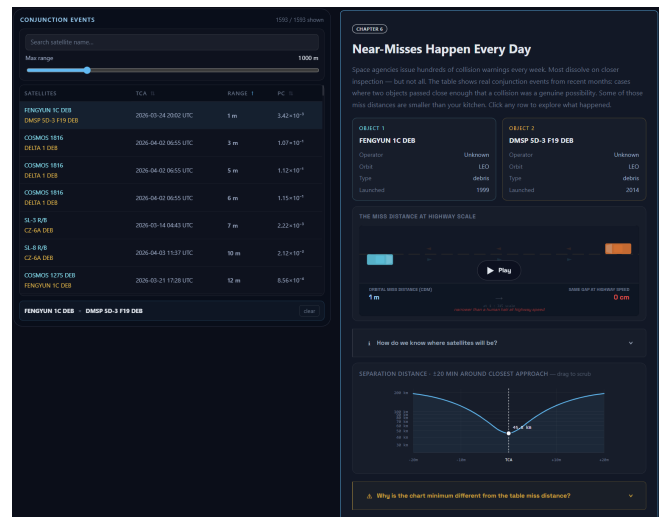
Figure 12. Chapter 6 — Near-Misses Happen Every Day . The most faithful adaptation of the original sketch: real SpaceTrack CDMs, an animated approach driven by browser-side SGP4, and a distance-vs-time plot.
