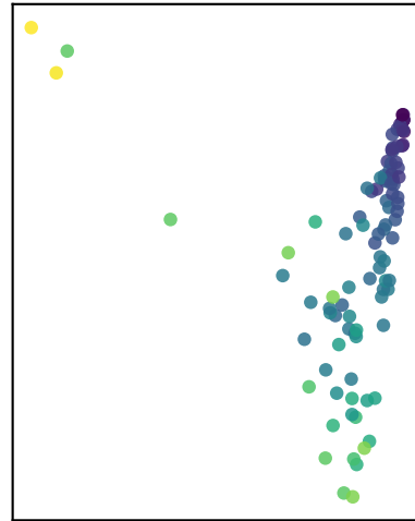
P2 (99 nodes)
