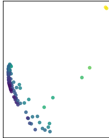
P3 (100 nodes)
