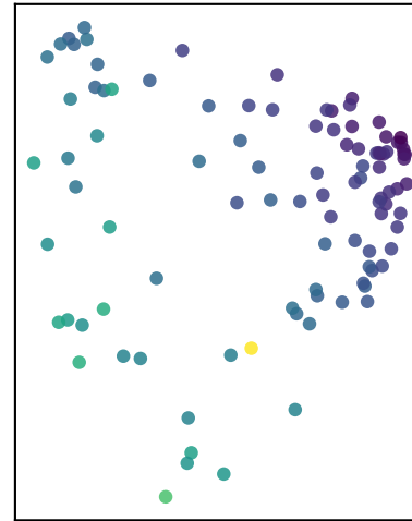
P4 (100 nodes)
