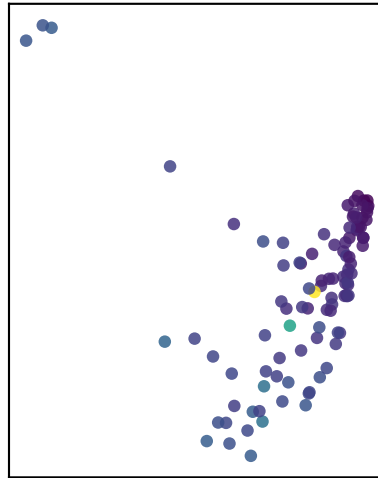
P1 (100 nodes)
