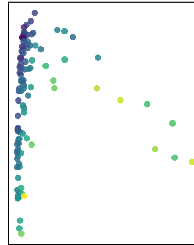
P5 (100 nodes)
