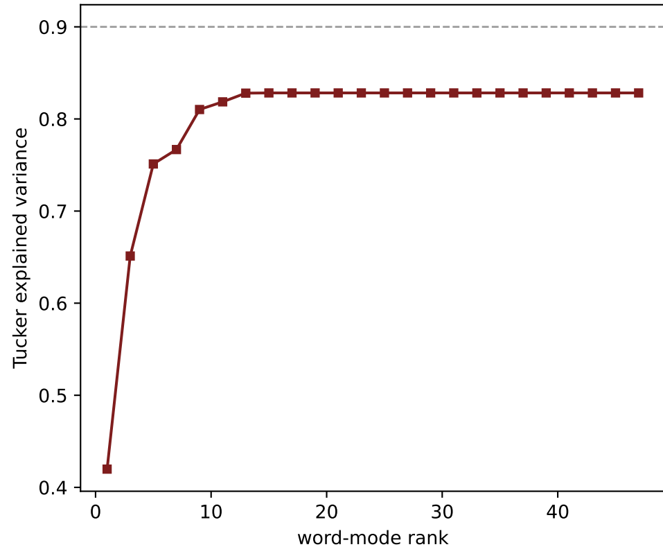
(c) Tensor-network compressibility (HOSVD)
