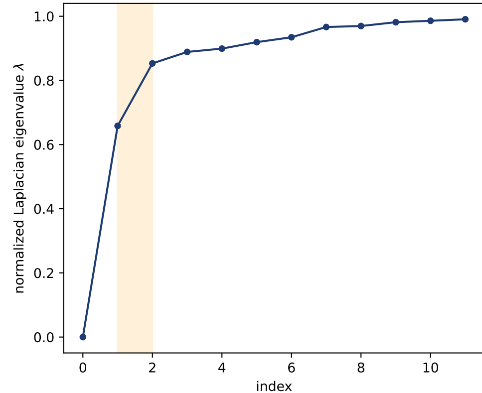
(a) Spirit-manifold spectrum (gap=0.195, eff.modes=10.9)
