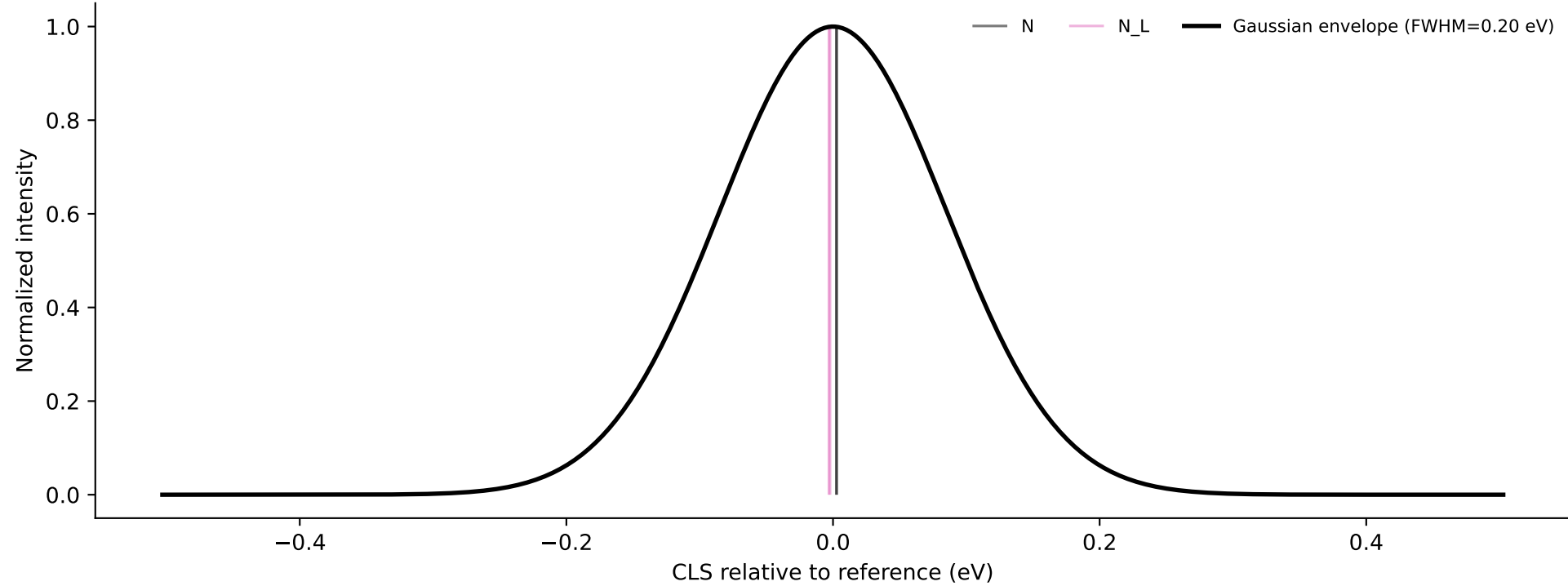
Planar molecule: N 1s initial-state shifts
