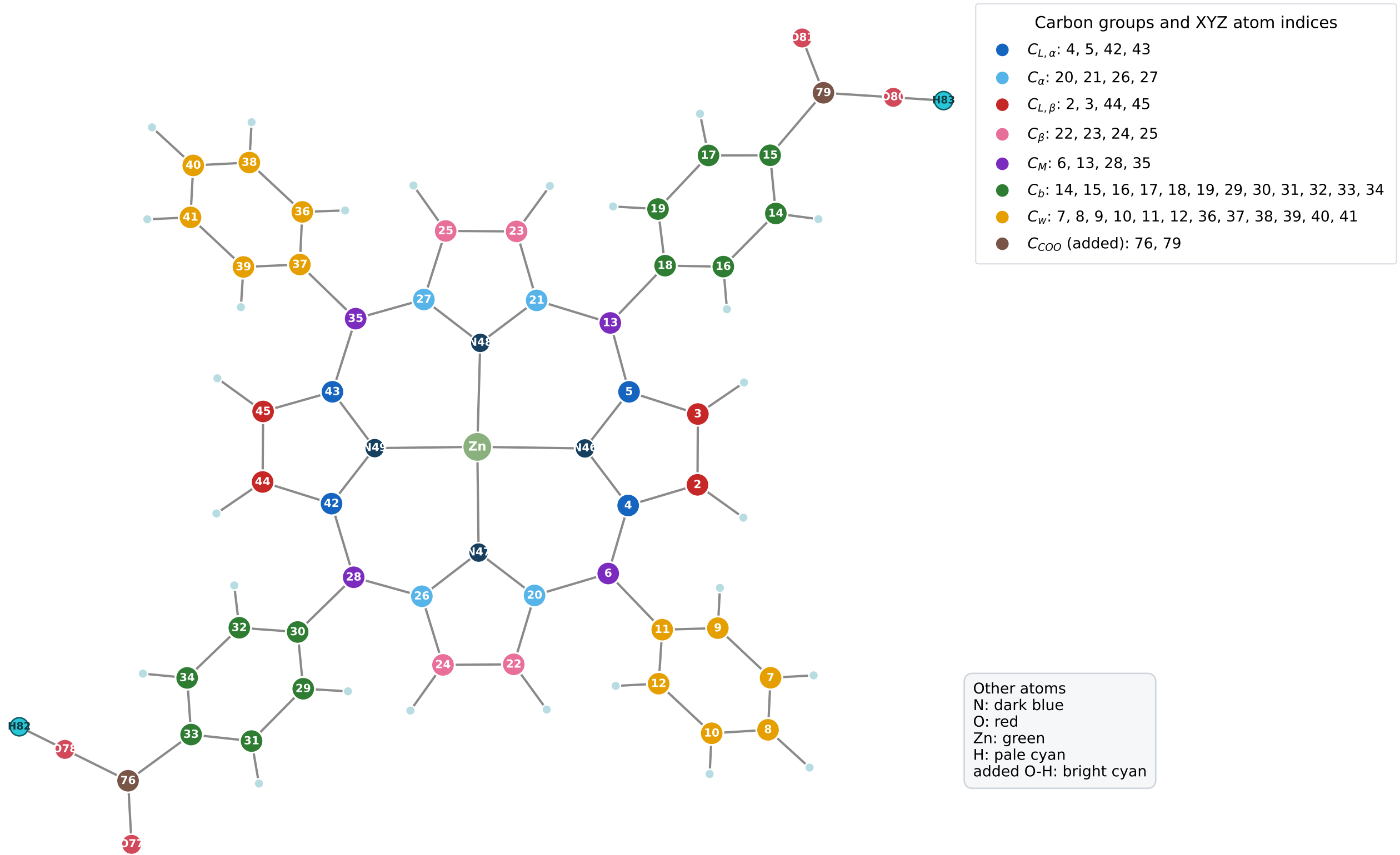
Two COOH groups: H82 is bonded to O78 and H83 is bonded to O80 (O-H = 0.98 Å).
