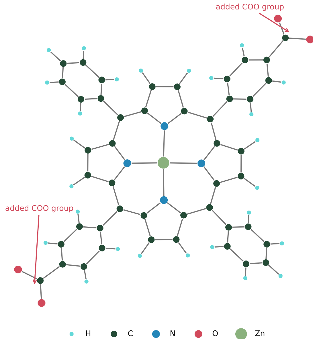
PLDC C46H26N4O4Zn1
