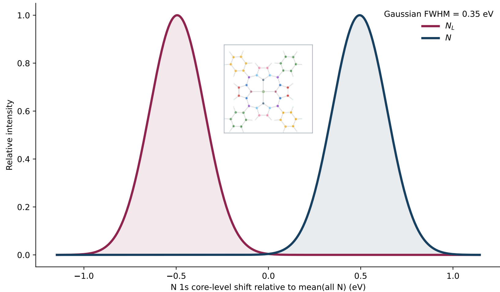
twistedH2: N 1s initial-state core-level shifts
