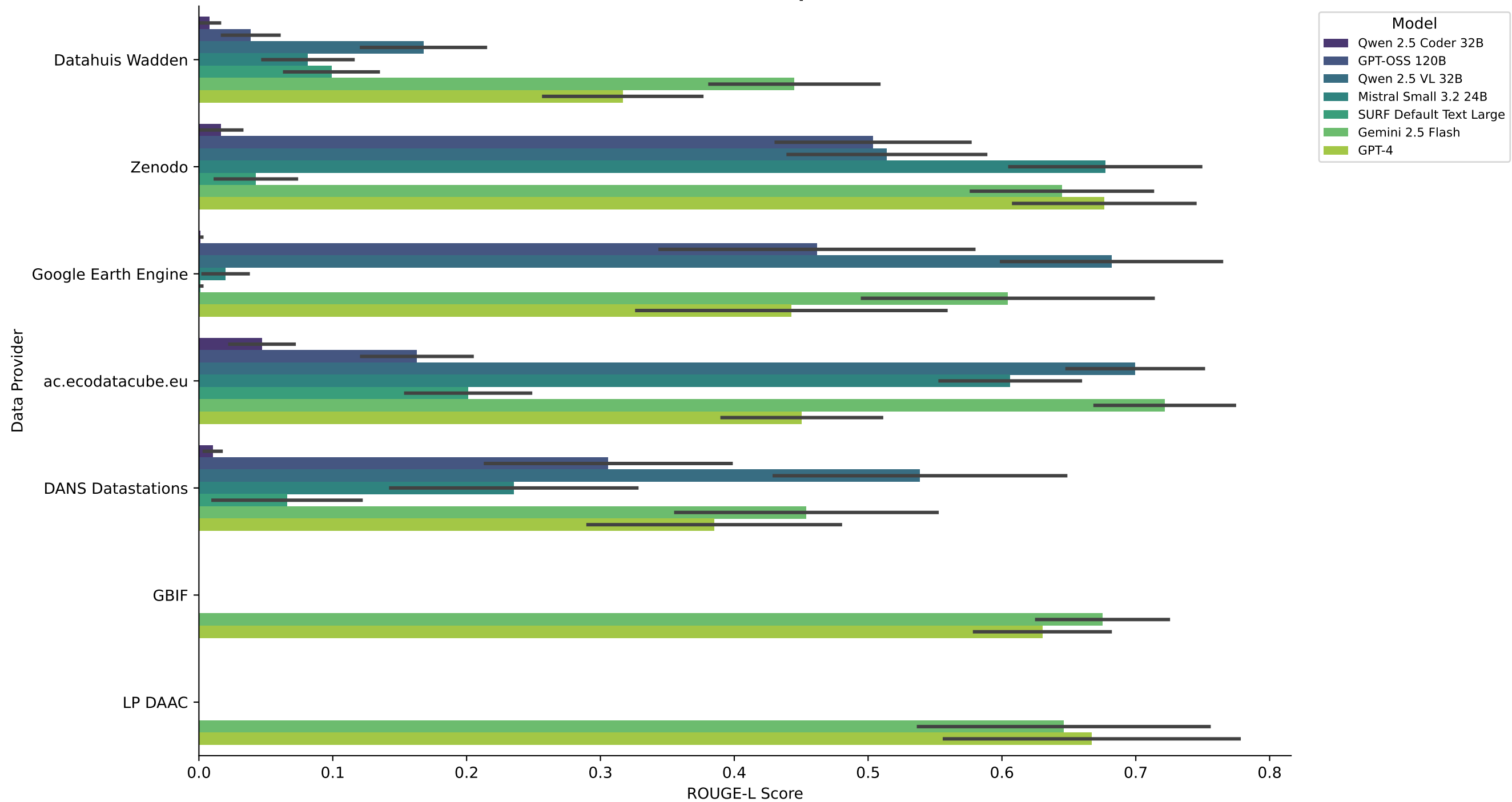
Retrieval Accuracy by Data Provider and Model (SURF, Gemini, OpenAI)
