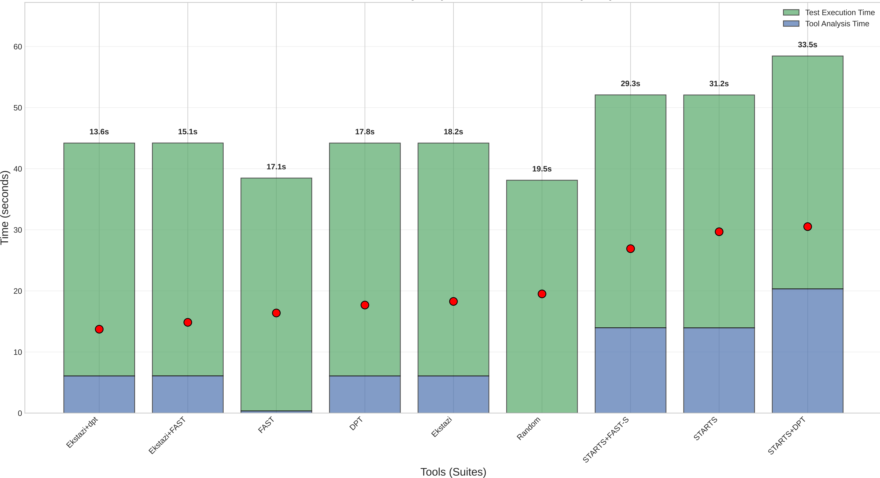
Test Execution Analysis (Median across ALL Projects)
