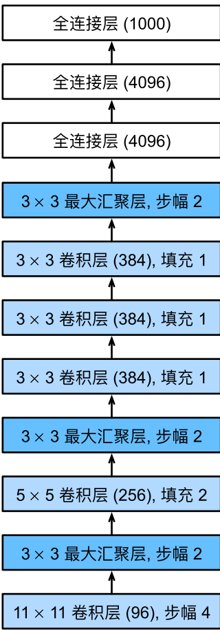
AlexNet
