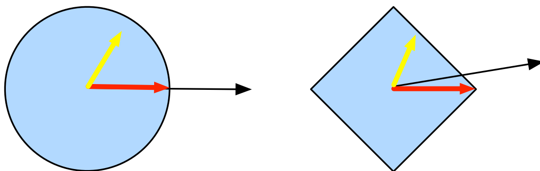
图 11.2.4 Convex Projections.
