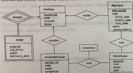
Fig. 2 E-R diagram
