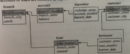
Fig.1 Schema diagram for the Banking database
