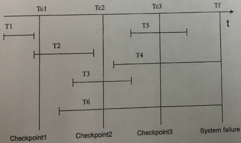
Fig.4 Concurrent schedule of transactions
