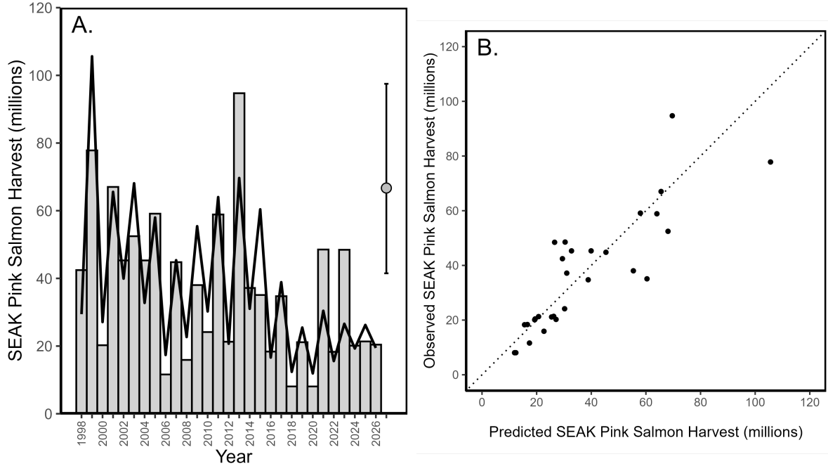
Figure 1: A. SEAK pink salmon harvest (millions) by year with the model fit (line) based upon the best performing model (model m2a). The predicted 2027 forecast (66.7 million fish) is symbolized as a grey circle with an 80% prediction interval (41.5-97.5 million fish). B. SEAK pink salmon harvest (millions) against the fitted values from model m2a by year. The dotted line is a one to one reference line.
