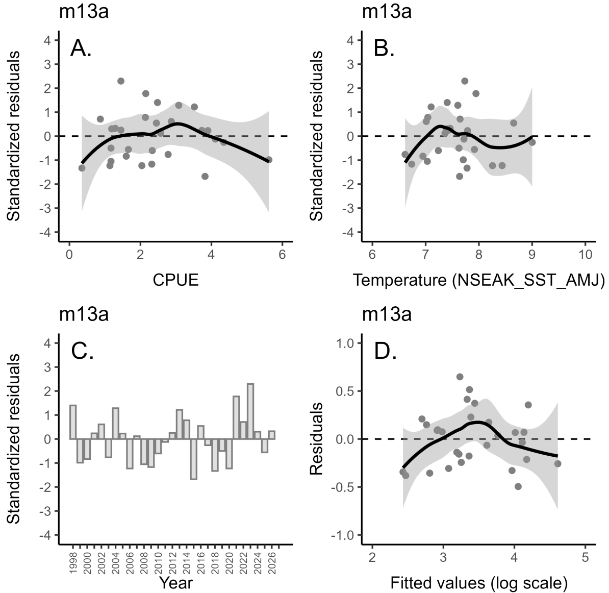
Figure C2: Standardized residuals versus predicted plots for A. CPUE and B. temperature (average April, May, June SST in northern Southeast Alaska) for model m13a. C. Standardized residuals versus juvenile year, and D. residuals versus fitted values for model m13a. Positive residuals indicate that the observed harvest was larger than predicted by the model.
