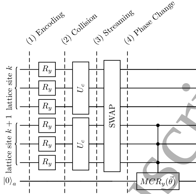
Figure 5. QLBM circuit, using the MCRY gate to store phase change data from the boundary lattice site. Circuit symbols: R_y are Y-rotation gates; U_c is the unitary collision operator; C denotes control qubits; and MCR_y(\vec{\theta}) is the multi-controlled rotation gate for phase change detection.
