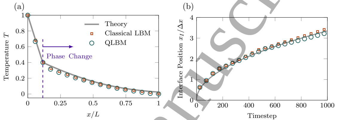
Figure 7. Comparison between the analytic solution, classical LBM, and quantum LBM (this work) methods. (a) Temperature distribution after 300 time steps, equivalent to t = 300 . The vertical dashed line indicates the interface location as predicted by theory. (b) Interface position evolution. The interface position is determined by the current melting node along with the liquid fraction at that node.
