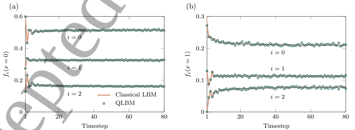
Figure 6. Time evolution of LBM distribution function values at (a) the left boundary and (b) the phase interface. Distributions f_i along different lattice directions i are shown as labeled. We limit this to the initial phase ( t \in [0, 80] ) to demonstrate the settling effect and quasi-static behavior.
