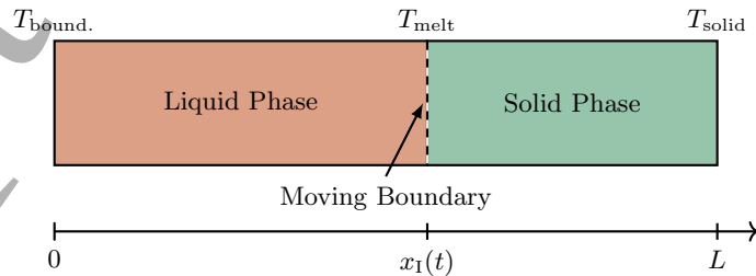
Figure 1. Schematic of a 1D phase change problem with a moving interface boundary. The domain of length L contains liquid (left) and solid (right) phases separated by a moving boundary at x_1(t) . This setup illustrates the Stefan problem for melting processes.
