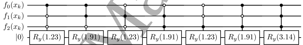
Figure 4. MCRY circuit evaluates possible measurement combinations at each lattice node, shown for the distributions f_i , by rotating the ancilla qubit. Rotation angles are determined by the sum S of control values.
