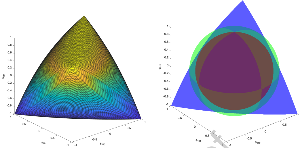
Figure 9: Boundary of moment space for s_{110} , s_{101} , and s_{011} where |J_1| = 0 . It has the form of a “puffy” regular tetrahedron centered at the origin. Left: complete surface. Right: a sphere of radius \sqrt{3}/4 (red) touches the boundary (blue) at one point on each face (e.g., 1/2, -1/2, 1/2 ). Outside the unit sphere (green), 0 \leq s_{110}s_{101}s_{011} on the boundary. Crossing jets (i.e., the VDF is two delta functions) correspond to one of the four extreme corner points where s_{110}s_{101}s_{011} = 1 . On the six edges connecting the corners where one of the cross moments equals \pm 1 , the VDF is positive on a 1D line in 3D phase space. Elsewhere on the four faces between the edges, the VDF is positive on a 2D surface in 3D phase space.
