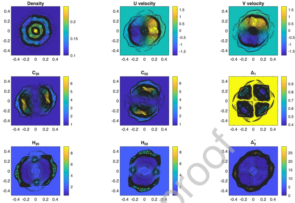
Figure 6: Ma = 4 , Kn = 0.1 , t = 0.05 . Low-order moments and Hankel determinants.
