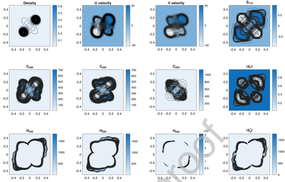
Figure 10: Impinging jets with Ma = 70 and Kn = 1 at t = 0.004 . Contour plots of lower-order moments. Regions where |\Delta_1| \approx 0 correspond to edges with s_{110} = \pm 1 .
