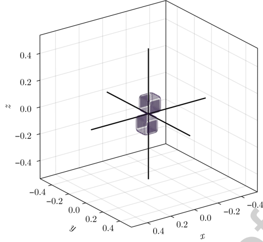
Figure 12: Initial condition for density with 3D jets. Inside the two cubes \rho = 1 , while outside \rho = 0.01 . For \text{Ma} = 3 , the velocity of the cubes is pointed towards the center (i.e., direction vectors (-1, -1, 1) and (1, 1, -1) ) and null otherwise. All other initial conditions are the same as in 2D.
