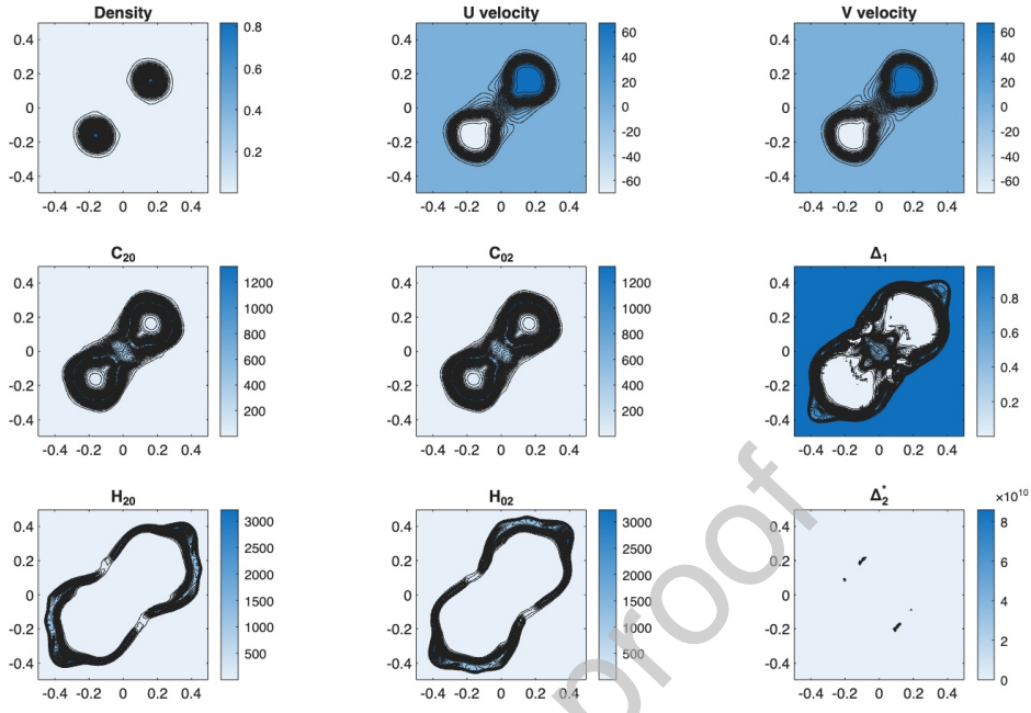
Figure 7: Crossing jets with Ma = 100 and Kn = 1000 at t = 0.003 . Low-order moments and Hankel determinants.
