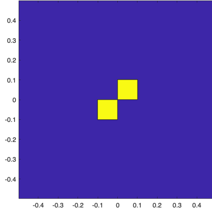
Figure 1: Initial conditions in the 2D computational domain. Unless stated otherwise, the dimensionless density m_{00} = 1 on the two central squares and 0.1 elsewhere. The other velocity moments are joint Gaussian with unit variances, and the correlation coefficient s_{11} is either 0 or \pm 1 . In the low-density region, the dimensionless mean velocity is found from m_{10} = m_{01} = 0 , while in the high-density squares m_{01} = m_{10} = \pm Ma / \sqrt{2} where in the lower square it is positive and in the upper square it is negative. Setting Ma = 0 results in a pressure-driven flow; otherwise, impinging/crossing jets correspond to large Ma .
