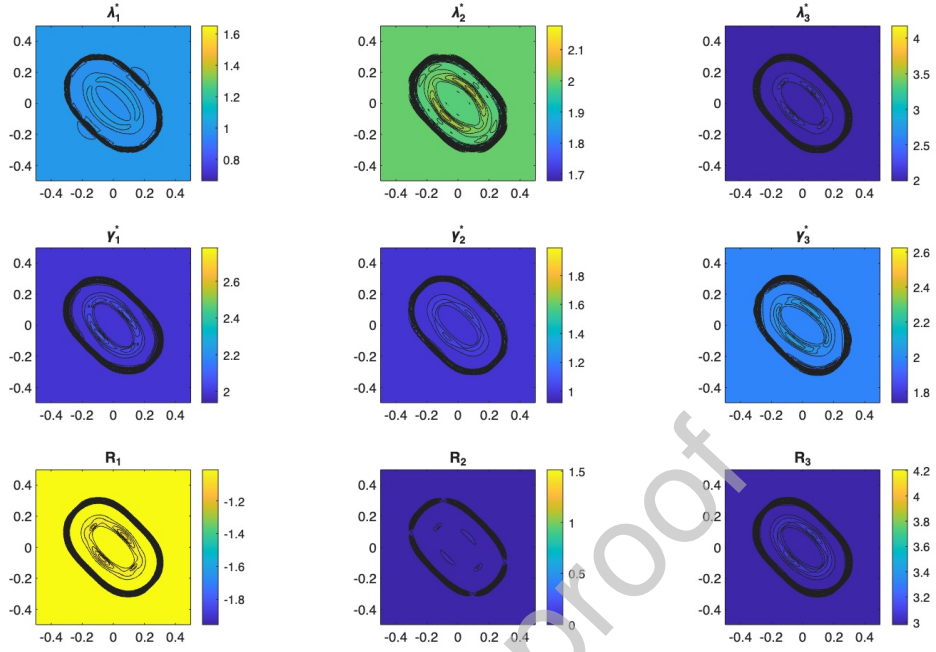
Figure 4: Ma = 4 , Kn = 0.001 , t = 0.05 . Realizability of \Delta_2^* . Top row: eigenvalues. Middle row: Cholesky diagonal elements. Bottom row: roots of the polynomial.
