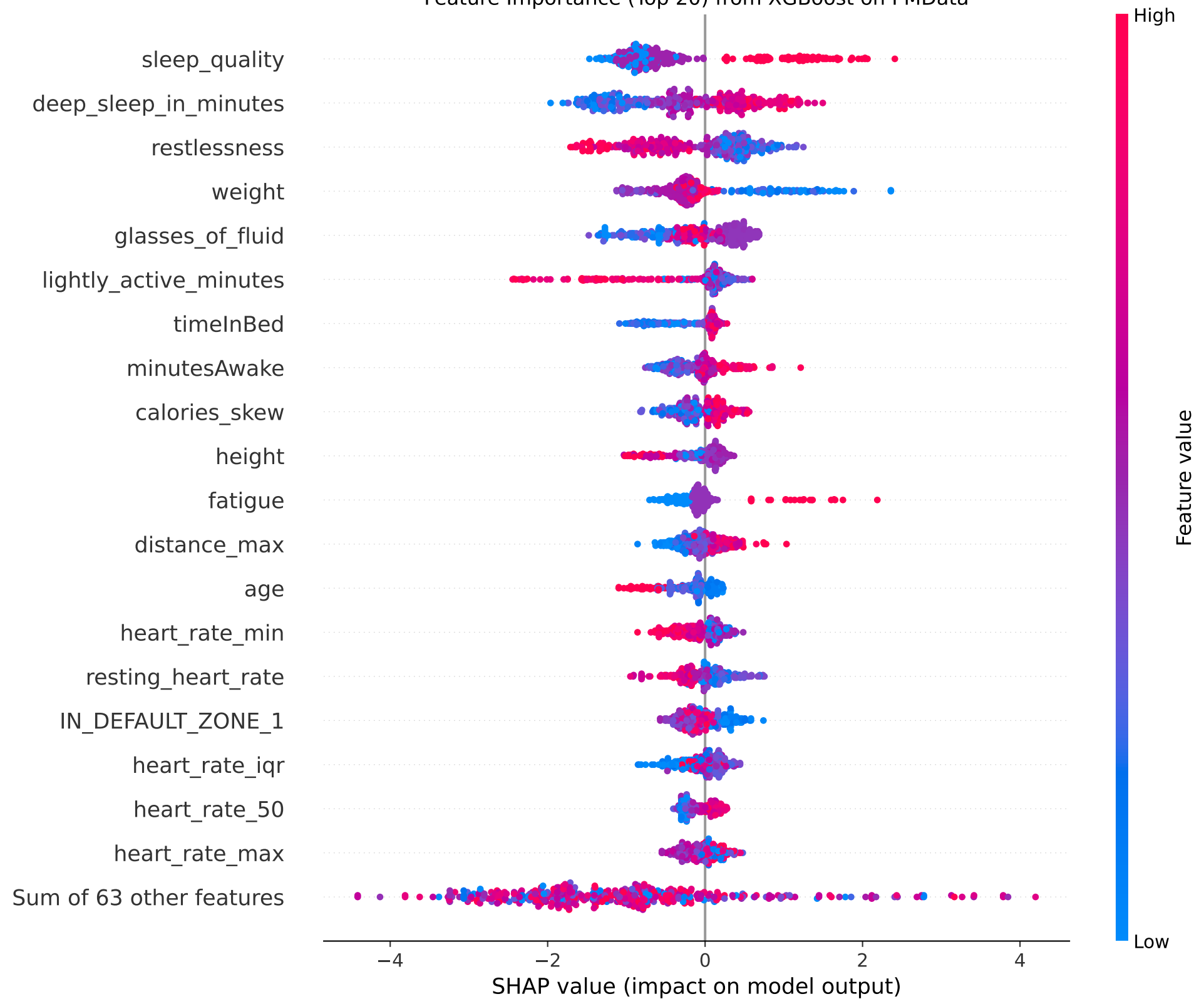
Feature Importance (Top 20) from XGBoost on PMData
