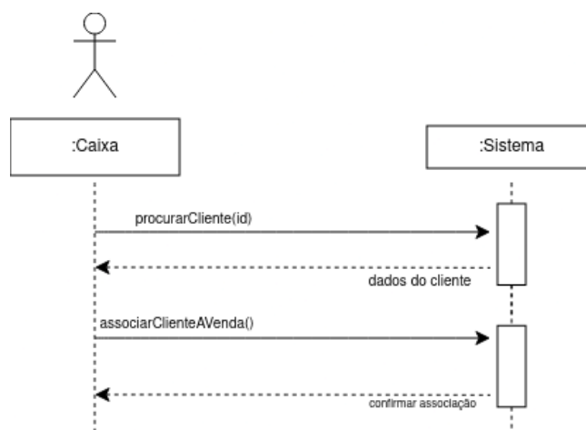
Fig. 14. UC11: Associar CLIENTE
