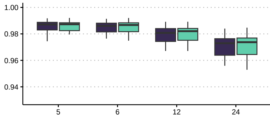
Minimum Count: 100
