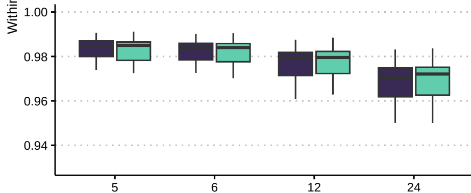
Minimum Count: 50
