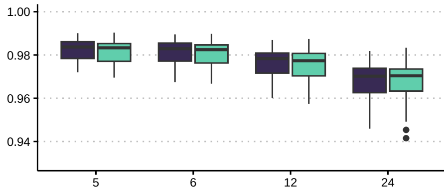
Window Size
