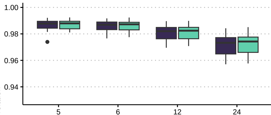
Minimum Count: 50
