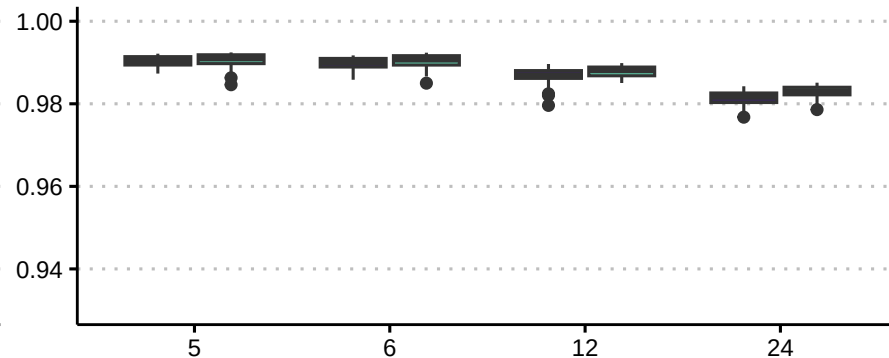
Cues: Migration
