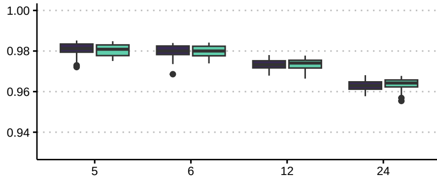
Cues: Environment
